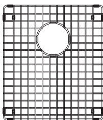
BGZ15S 16" x 13 7/8" x 1" 406 x 352 x 25 mm FUN#112.0194.710
