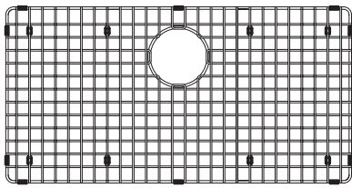
BG210S 13 5/8" x 26 11/16" x 1" 346 x 678 x 25 mm FUN#112.0055.042
