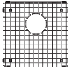
BGDS15S 14 1/4" x 14 1/4" x 1" 362 x 362 x 25 mm FUN#112.0054.949
