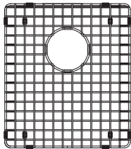
BGDS14S 15 1/4" x 13 1/4" x 1" 387 x 337 x 25 mm FUN#112.0078.322
