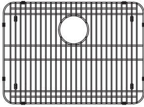
BGA2317S 15" x 21" x 1" 381 x 533 x 25 mm FUN#112.0174.875
