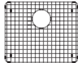
BG14S 15" x 18" x 1" 381 x 457 x 25 mm FUN#112.0486.240
