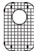
BG35S 14 1/4" x 8 1/2" x 1" 362 x 216 x 25 mm FUN#112.0044.796
