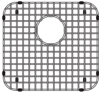
BG11S 14 1/4" x 15 1/4" x 1" 362 x 387 x 25 mm FUN#112.0044.786
